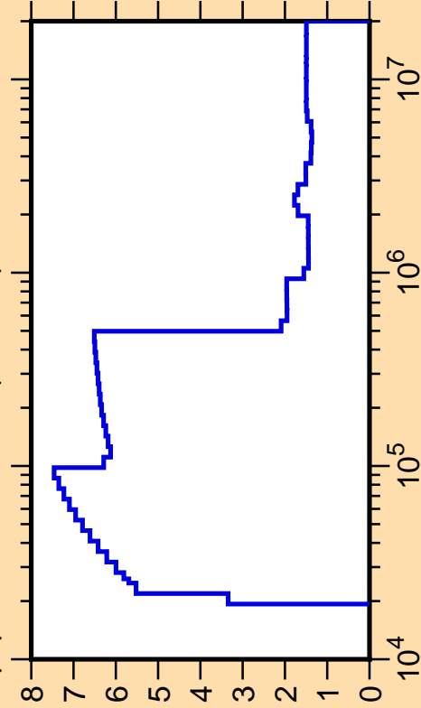
\Delta\mu/\mu vs. E for ^{34}\text{Cl}(\text{mt251})
