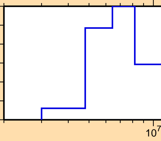
\sigma vs. E for ^{34}\text{Cl}(n,n\text{cont.})
