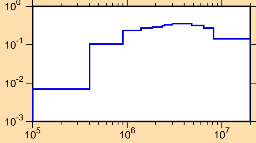
\sigma vs. E for ^{34}\text{Cl}(n,\text{inel.})
