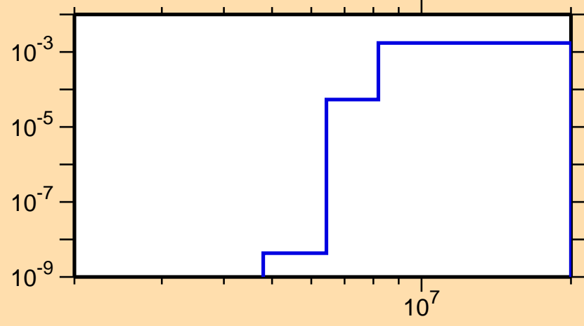
\sigma vs. E for ^{34}\text{Cl}(n,t)
