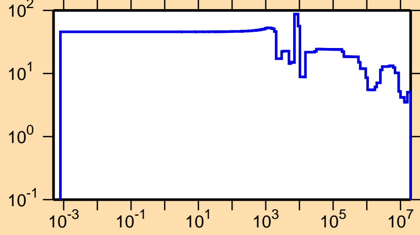
\Delta\sigma/\sigma vs. E for ^{34}\text{Cl}(n,\text{el.})
