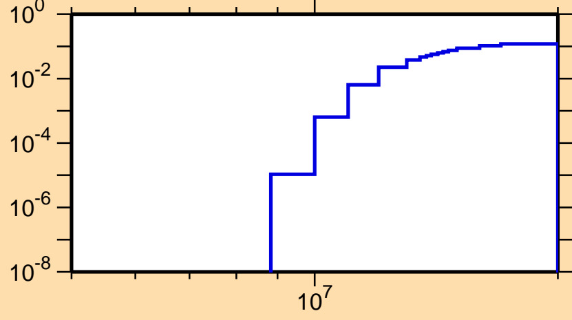
\sigma vs. E for ^{35}\text{Cl}(n,n\alpha)
