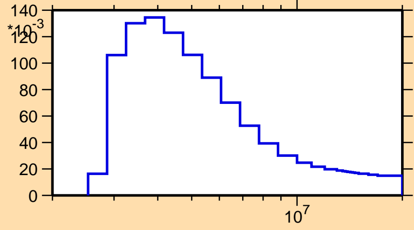
\sigma vs. E for ^{35}\text{Cl}(n,n_3)
