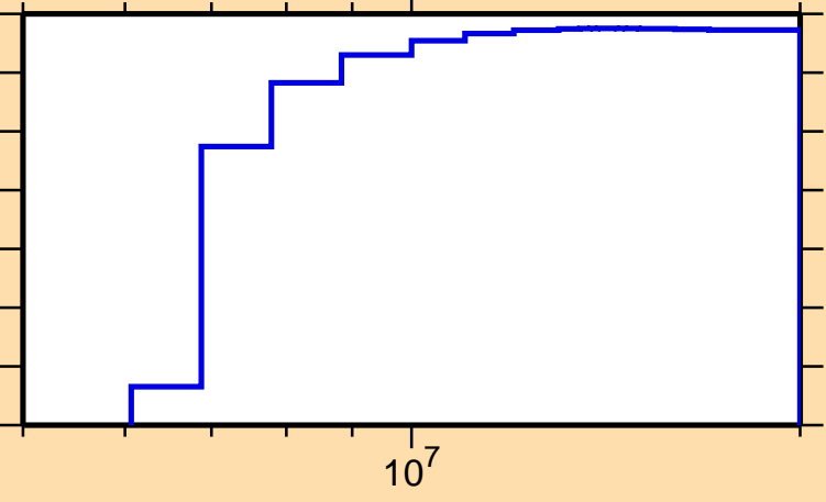
\sigma vs. E for ^{35}\text{Cl}(n,np)
