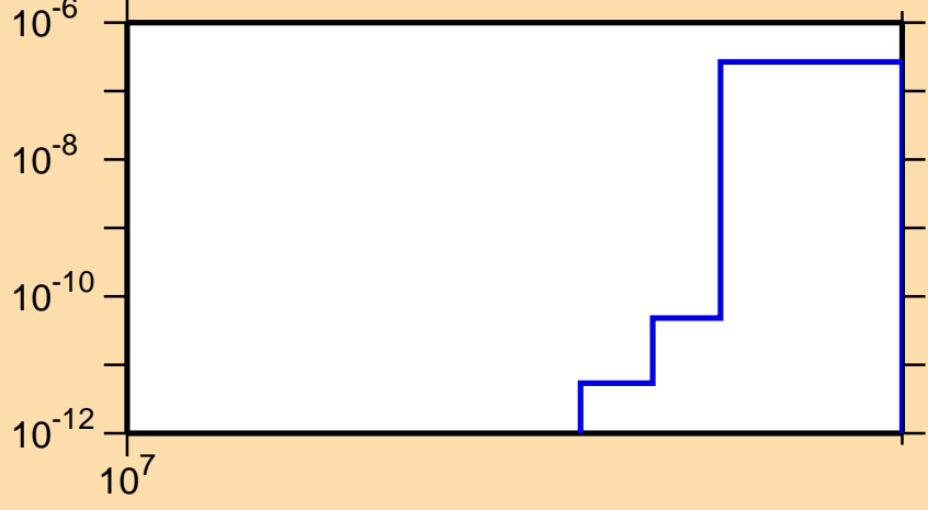
\sigma vs. E for ^{35}\text{Cl}(n,pd)
