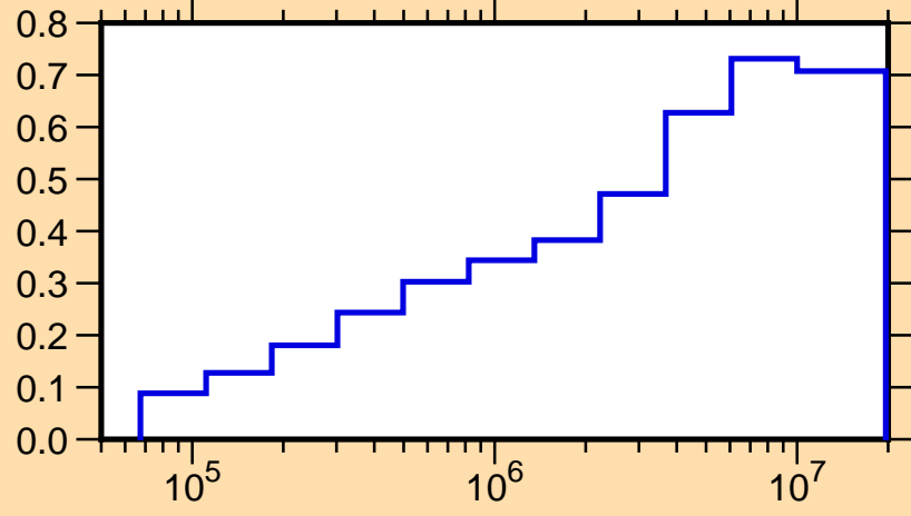
\mu vs. E for ^{35}\text{Cl}(\text{mt251})
