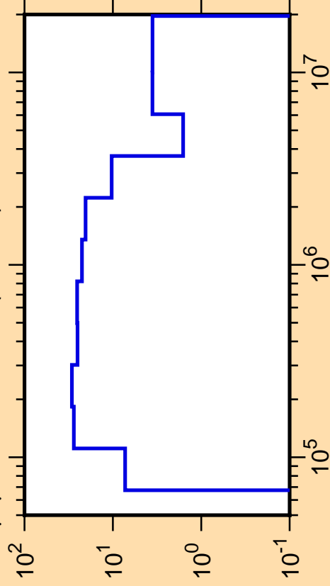
\Delta\mu/\mu vs. E for ^{35}\text{Cl}(\text{mt251})
