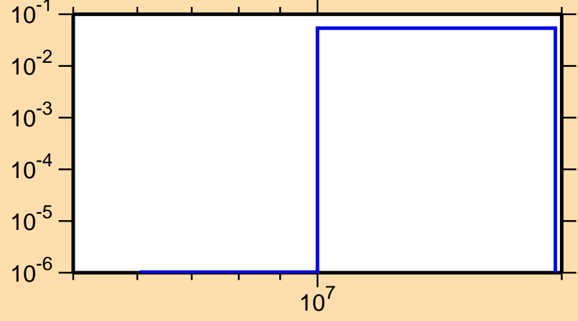
\sigma vs. E for ^{35}\text{Cl}(n,\alpha)
