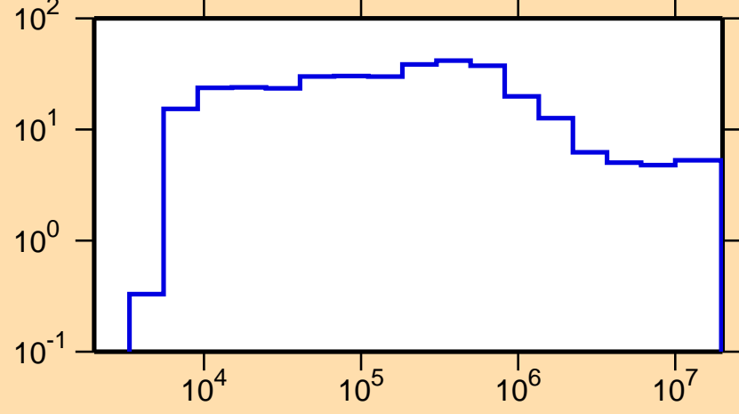
\Delta\sigma/\sigma vs. E for ^{35}\text{Cl}(n,\text{nonel.})
