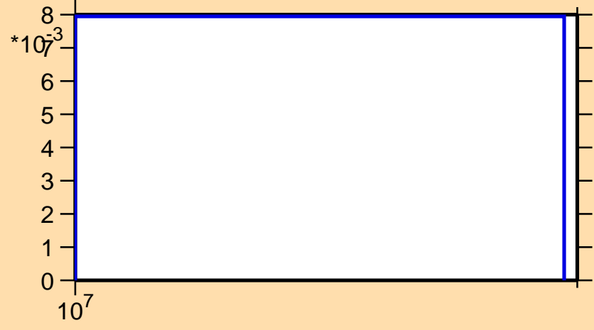
\sigma vs. E for ^{35}\text{Cl}(n,2n)
