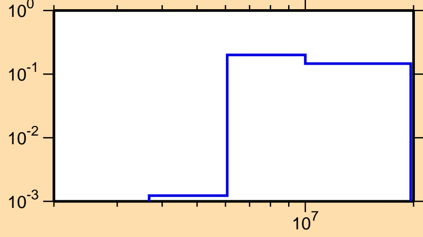
\sigma vs. E for ^{35}\text{Cl}(n,n\text{cont.})
