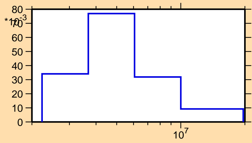
\sigma vs. E for ^{35}\text{Cl}(n,n_4)
