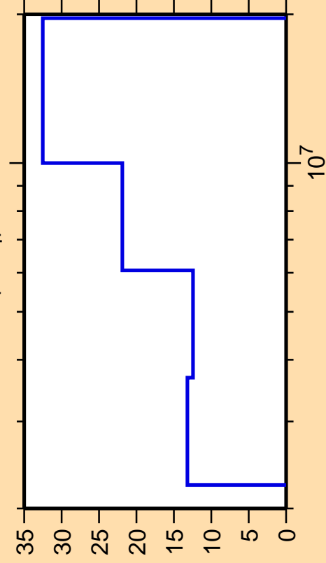
\Delta\sigma/\sigma vs. E for ^{35}\text{Cl}(n,n_4)
