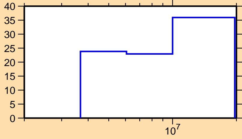
\Delta\sigma/\sigma vs. E for ^{35}\text{Cl}(n,ncont.)
