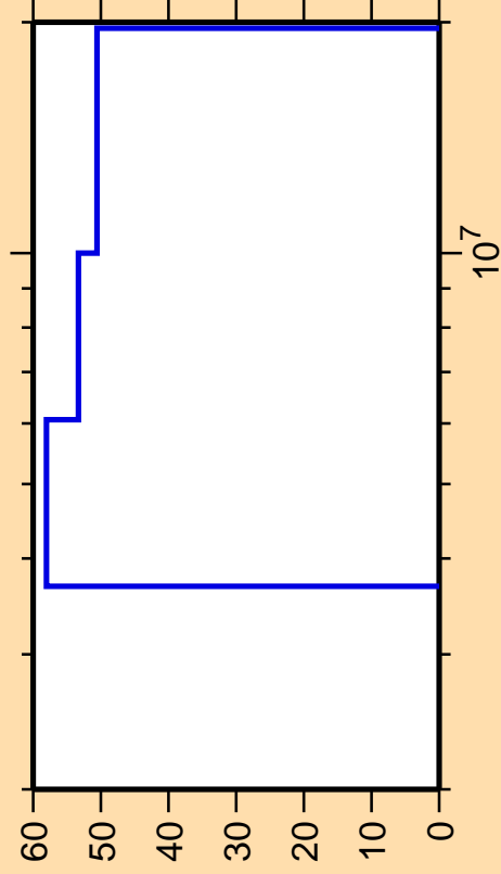
\Delta\sigma/\sigma vs. E for ^{35}\text{Cl}(n,d)
