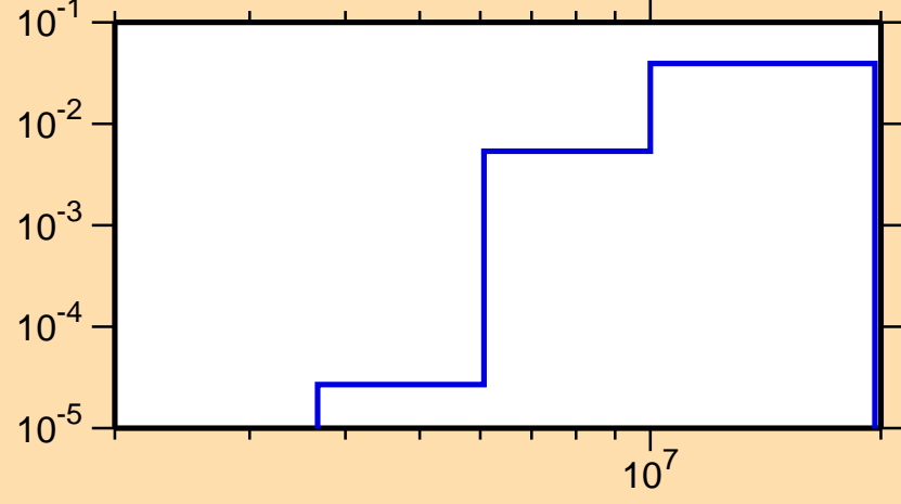
\sigma vs. E for ^{35}\text{Cl}(n,d)
