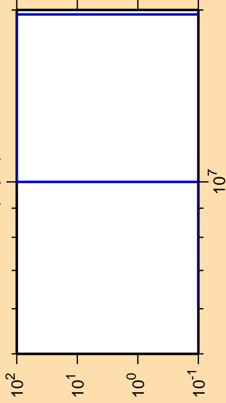
\Delta\sigma/\sigma vs. E for ^{35}\text{Cl}(n,p\alpha)
