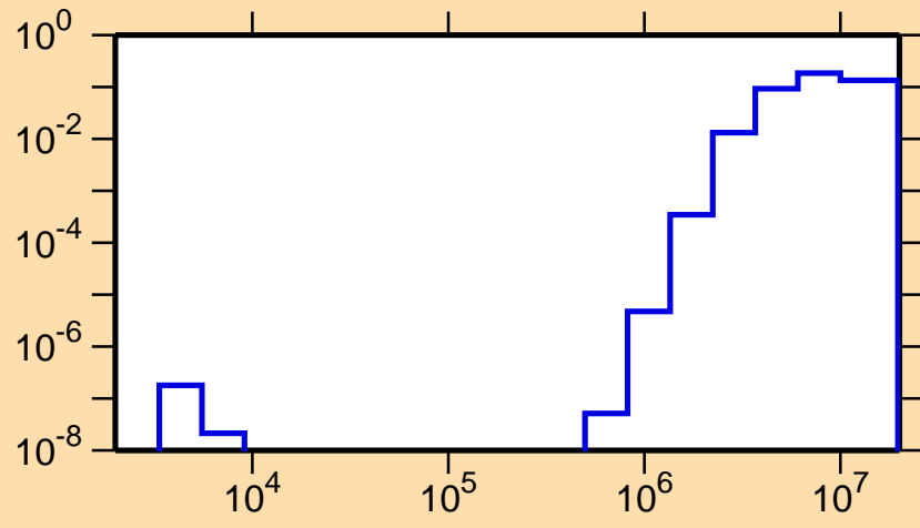
\sigma vs. E for ^{35}\text{Cl}(n,\alpha)
