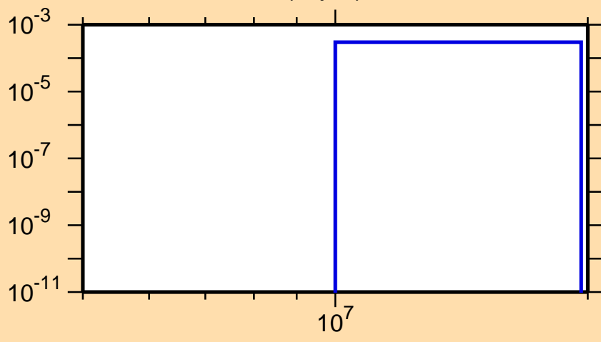
\sigma vs. E for ^{35}\text{Cl}(n,p\alpha)
