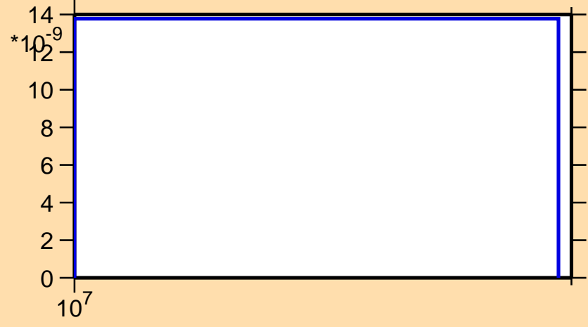
\sigma vs. E for ^{35}\text{Cl}(n,2np)
