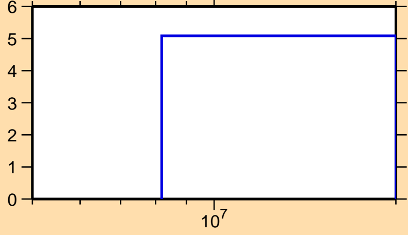
\Delta\sigma/\sigma vs. E for ^{35}\text{Cl}(n,\text{nonel.})
