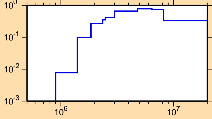
\sigma vs. E for ^{35}\text{Cl}(n,\text{inel.})
