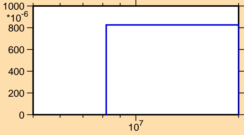
\sigma vs. E for ^{35}\text{Cl}(n,t)
