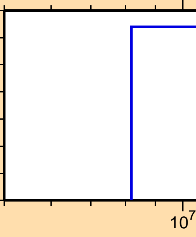
\sigma vs. E for ^{35}\text{Cl}(n,2n)
