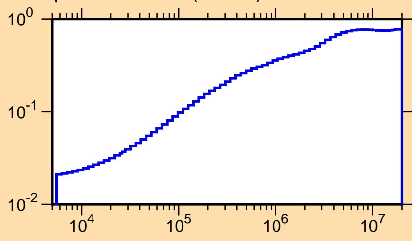
\mu vs. E for ^{36}\text{Cl}(\text{mt251})
