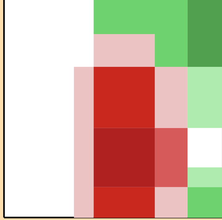
\Delta\sigma/\sigma vs. E for ^{36}\text{Cl}(n,2n)
