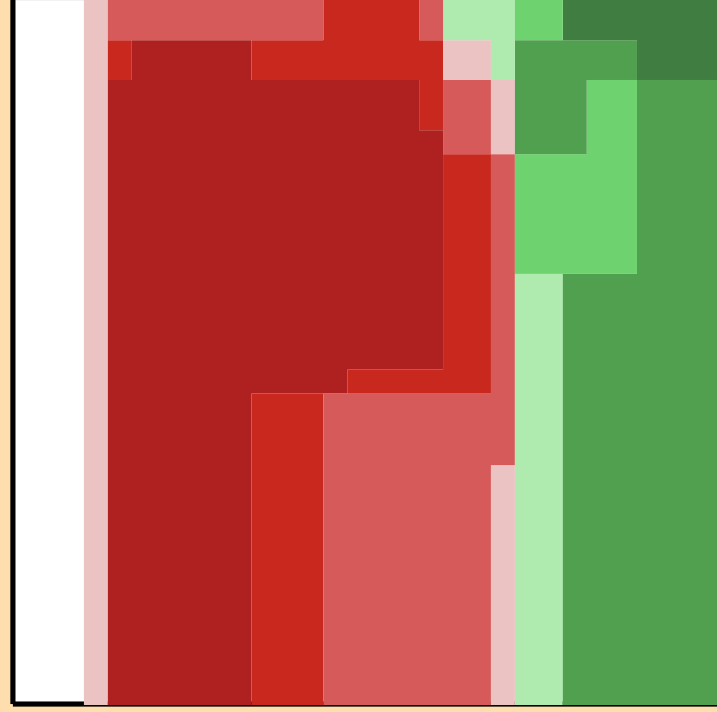
\Delta\sigma/\sigma vs. E for ^{36}\text{Cl}(n,\text{inel.})
