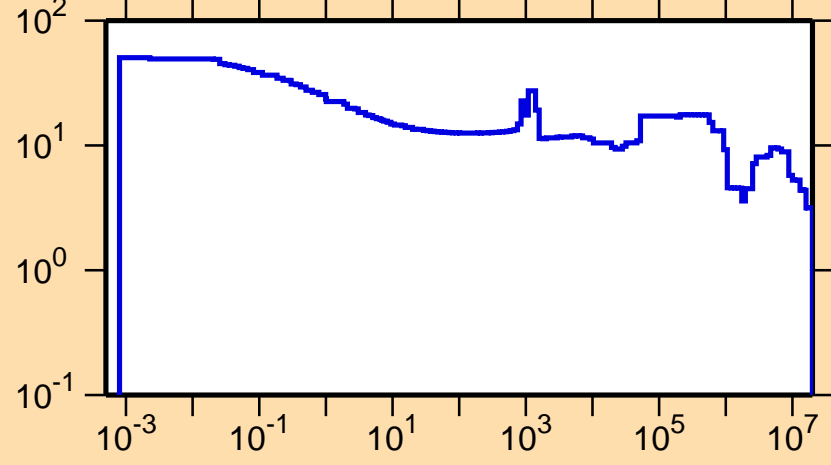
\Delta\sigma/\sigma vs. E for ^{36}\text{Cl}(n,\text{tot.})
