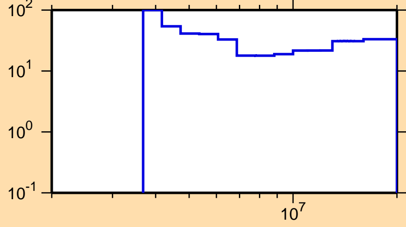
\Delta\sigma/\sigma vs. E for ^{36}\text{Cl}(n,n\text{cont.})
