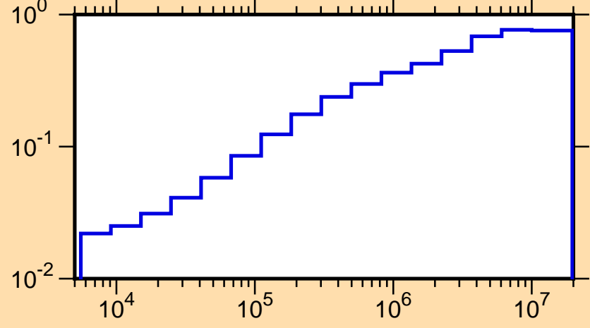
\mu vs. E for ^{36}\text{Cl}(\text{mt251})
