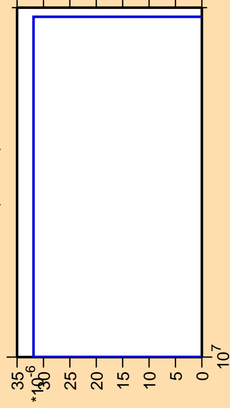
\Delta\sigma/\sigma vs. E for ^{36}\text{Cl} (mt 34)
