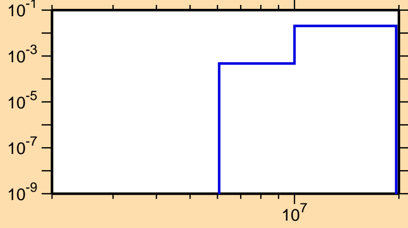
\sigma vs. E for ^{36}\text{Cl}(n,d)
