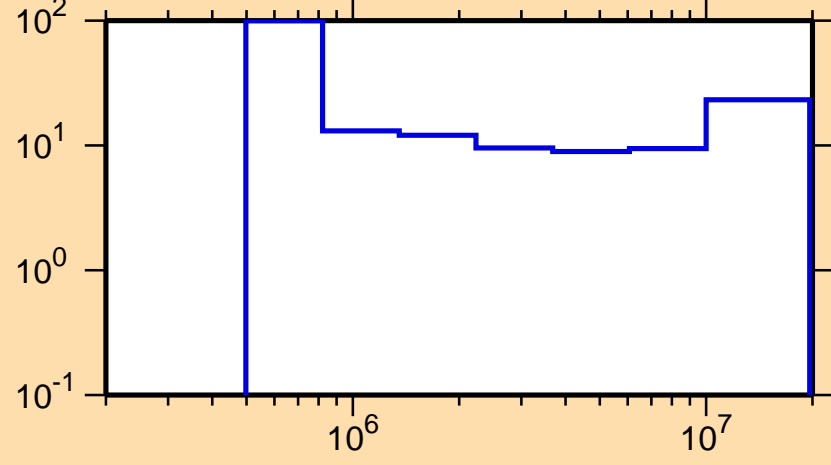
\Delta\sigma/\sigma vs. E for ^{36}\text{Cl}(n,\text{inel.})
