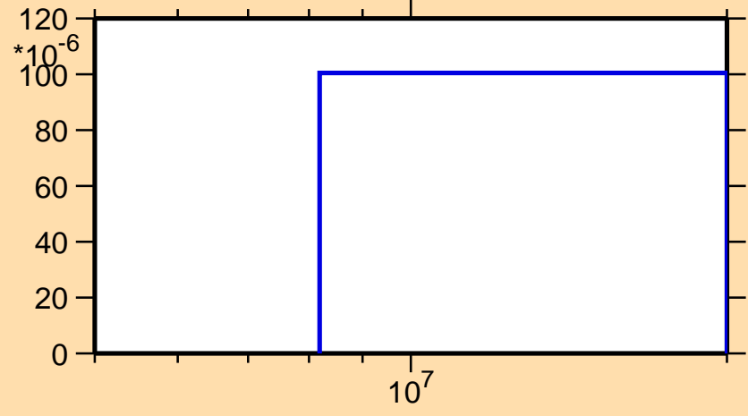
\sigma vs. E for ^{36}\text{Cl}(n,\text{nd})
