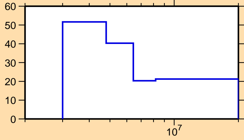
\Delta\sigma/\sigma vs. E for ^{36}\text{Cl}(n,ncont.)
