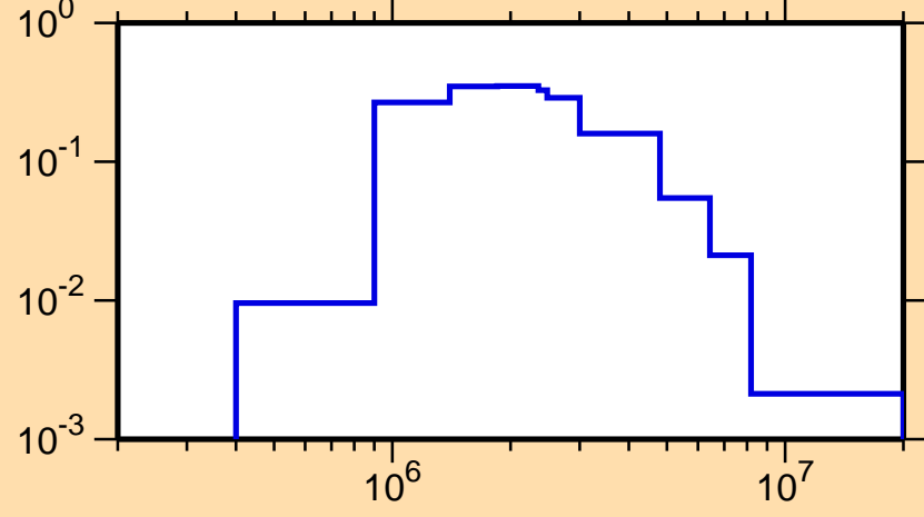
\sigma vs. E for ^{36}\text{Cl}(n,n_1)
