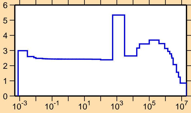
\sigma vs. E for ^{36}\text{Cl}(n,\text{el.})
