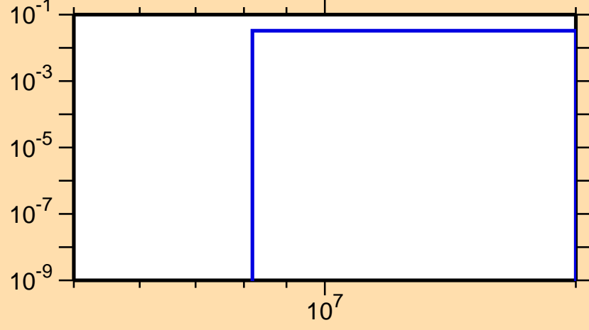
\sigma vs. E for ^{36}\text{Cl}(n,\alpha)
