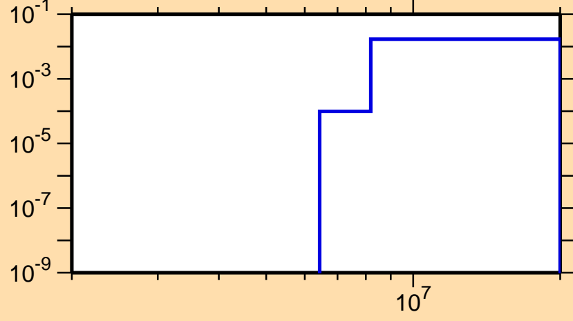
\sigma vs. E for ^{36}\text{Cl}(n,d)
