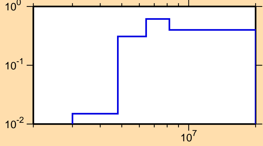
\sigma vs. E for ^{36}\text{Cl}(n,n\text{cont.})
