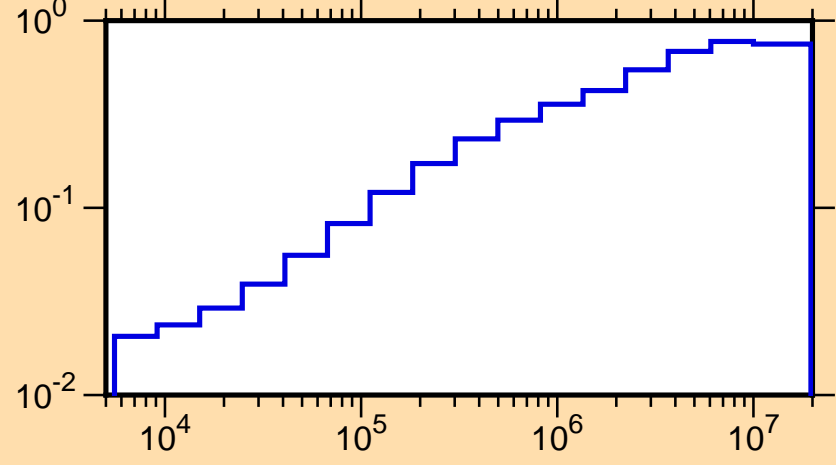
\mu vs. E for ^{38}\text{Cl}(\text{mt251})
