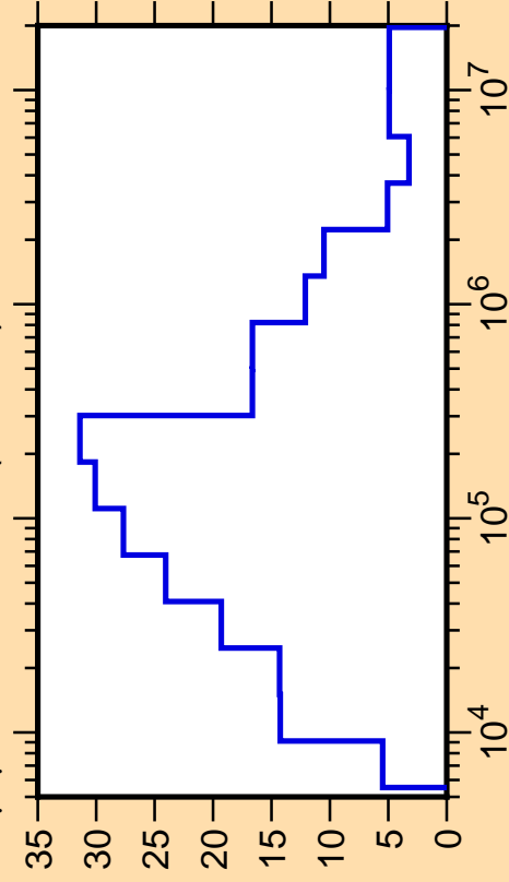
\Delta\mu/\mu vs. E for ^{38}\text{Cl}(\text{mt251})
