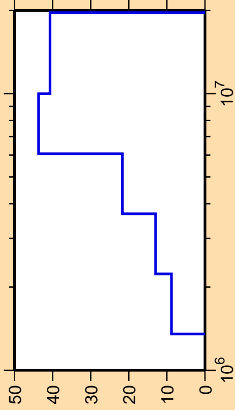
\Delta\sigma/\sigma vs. E for ^{38}\text{Cl}(n,n_4)
