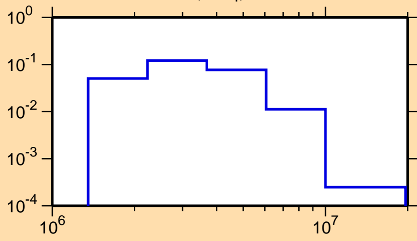
\sigma vs. E for ^{38}\text{Cl}(n,n_4)
