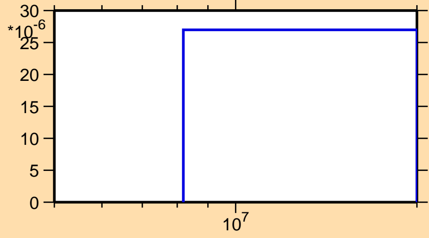
\sigma vs. E for ^{38}\text{Cl}(n,3n)
