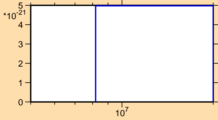
\sigma vs. E for ^{38}\text{Cl}(n,\text{pt})
