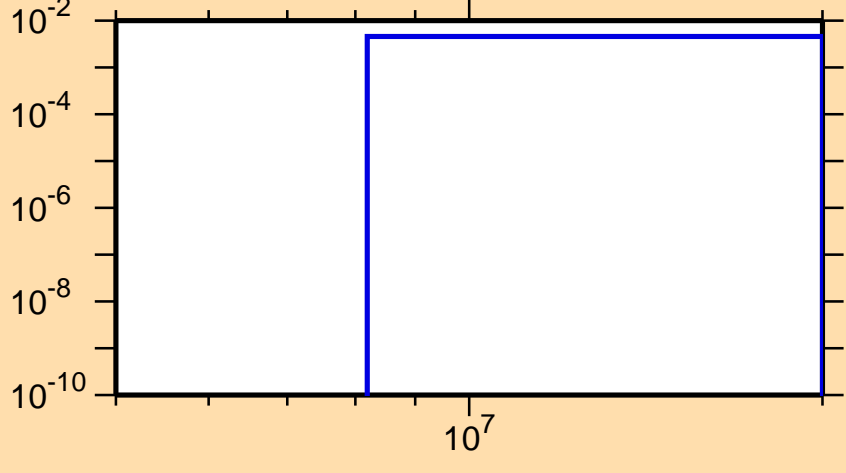
\sigma vs. E for ^{38}\text{Cl}(n,d)
