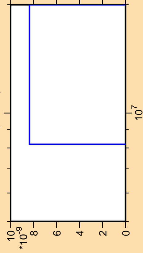
\Delta\sigma/\sigma vs. E for ^{38}\text{Cl}(\text{mt } 45)
