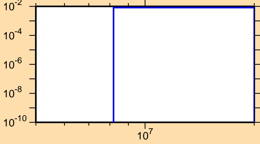
\sigma vs. E for ^{38}\text{Cl}(n,\alpha)
