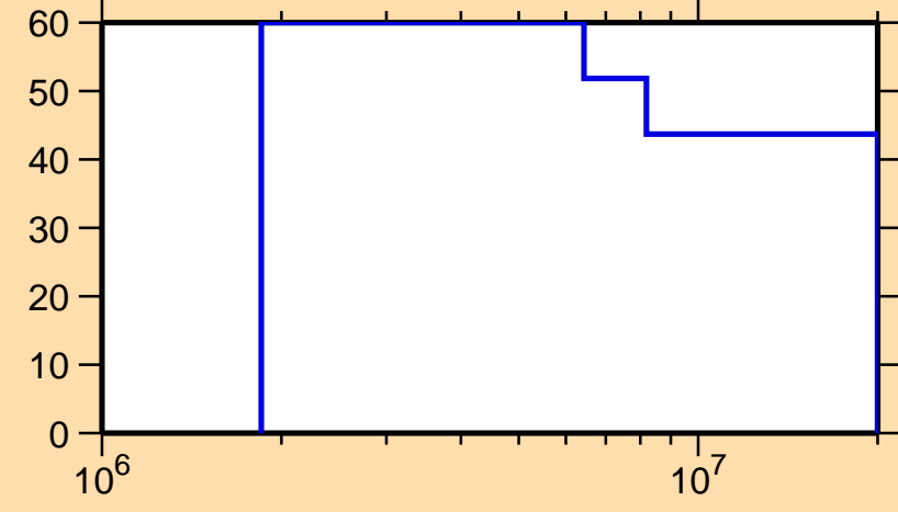
\Delta\sigma/\sigma vs. E for ^{38}\text{Cl}(n,p)
