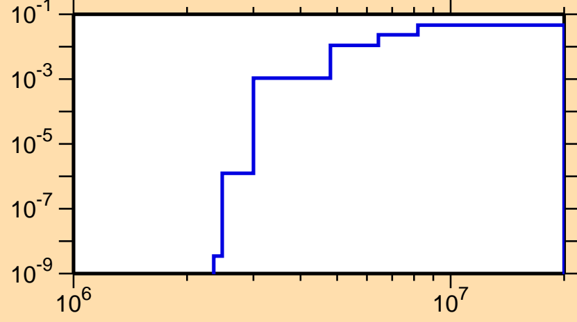
\sigma vs. E for ^{38}\text{Cl}(n,p)
