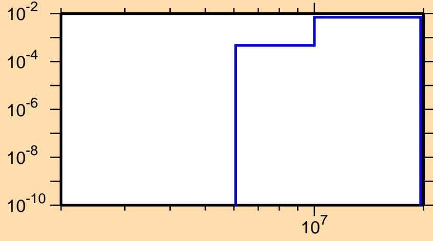
\sigma vs. E for ^{39}\text{Cl}(n,p)
