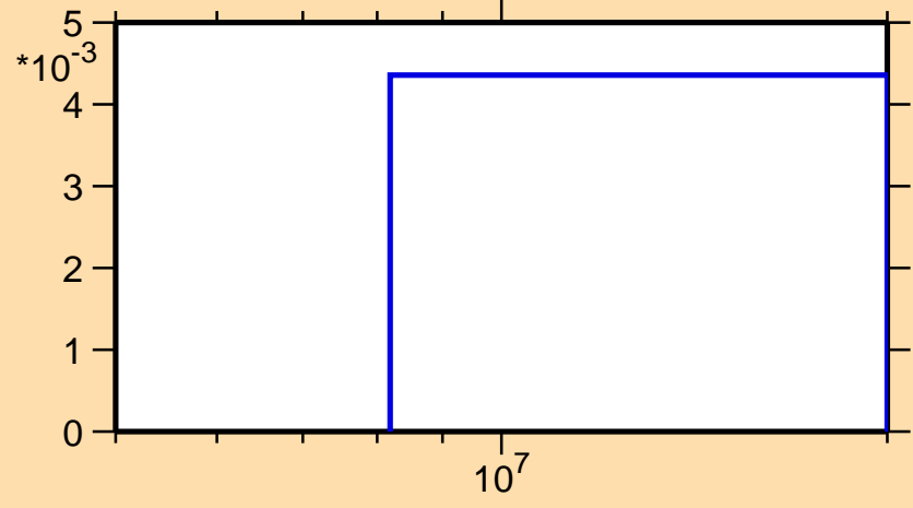
\sigma vs. E for ^{39}\text{Cl}(n,3n)
