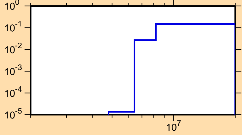
\sigma vs. E for ^{39}\text{Cl}(n,n\text{cont.})
