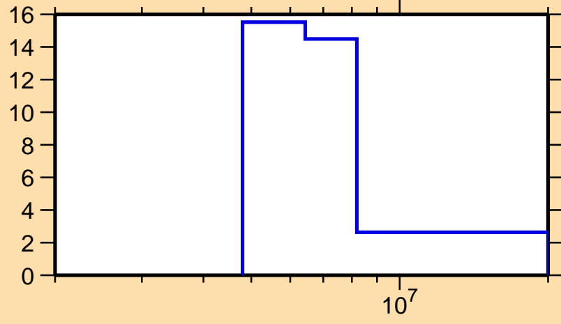
\Delta\sigma/\sigma vs. E for ^{39}\text{Cl}(n,el.)
