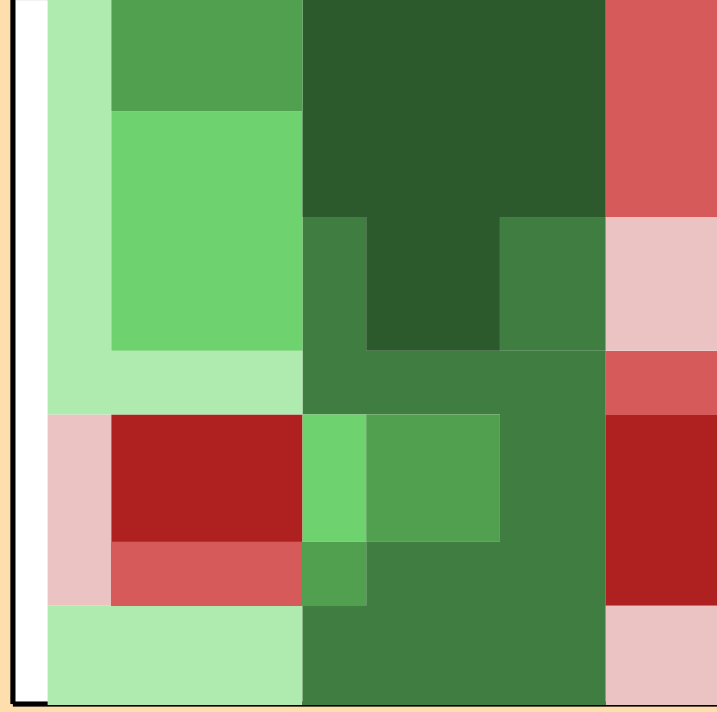
\Delta\sigma/\sigma vs. E for ^{40}\text{Cl}(n,2n)
