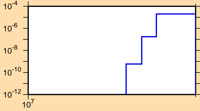
\sigma vs. E for ^{40}\text{Cl}(n,2n\alpha)
