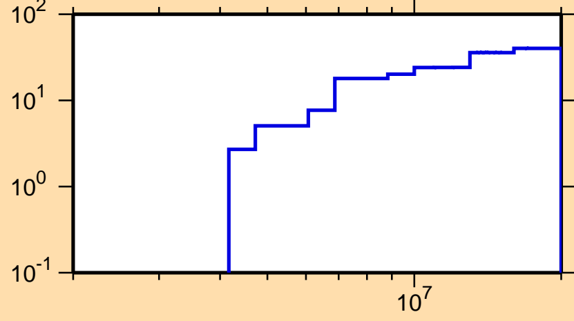
\Delta\sigma/\sigma vs. E for ^{40}\text{Cl}(n,\text{inel.})
