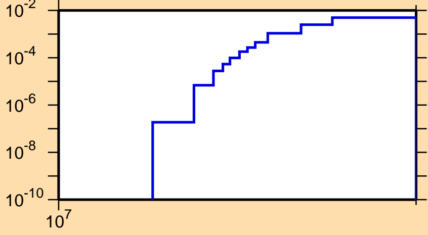
\sigma vs. E for ^{40}\text{Cl}(n,np)
