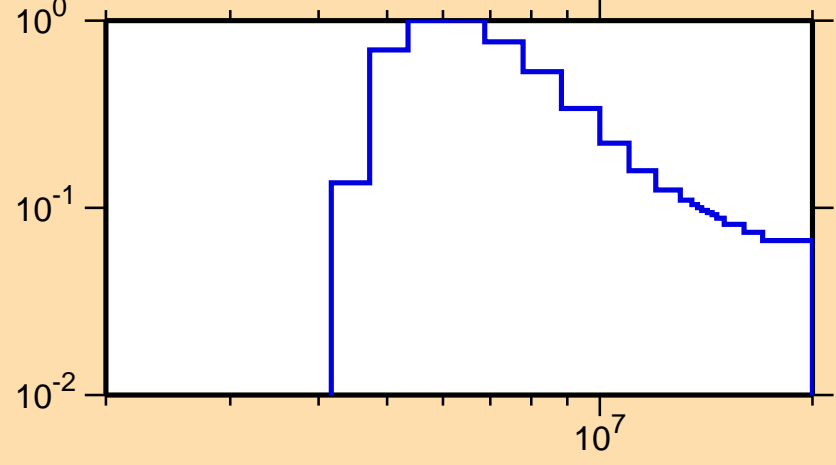
\sigma vs. E for ^{40}\text{Cl}(n,n\text{cont.})
