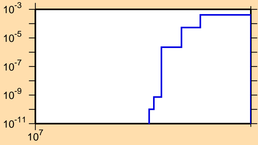
\sigma vs. E for ^{40}\text{Cl}(n,\text{nd})
