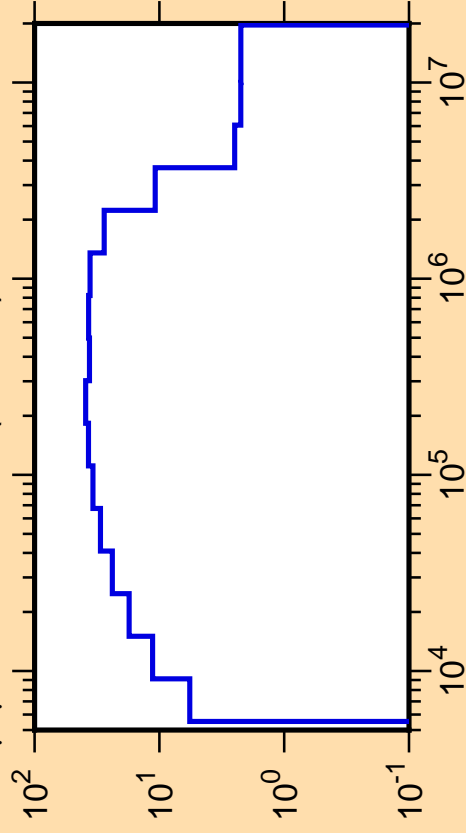
\Delta\mu/\mu vs. E for ^{40}\text{Cl}(\text{mt251})
