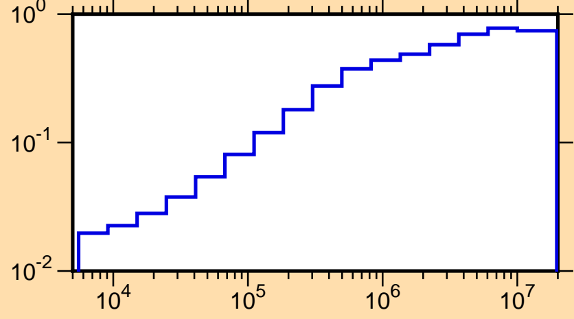
\mu vs. E for ^{40}\text{Cl}(\text{mt251})
