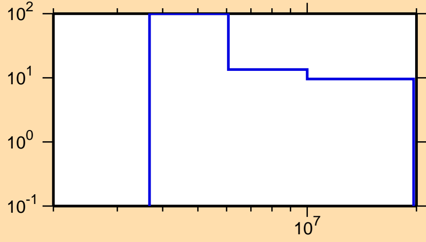
\Delta\sigma/\sigma vs. E for ^{40}\text{Cl}(n,2n)
