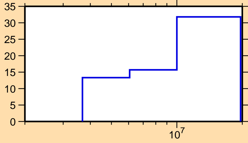
\Delta\sigma/\sigma vs. E for ^{40}\text{Cl}(n,n\text{cont.})
