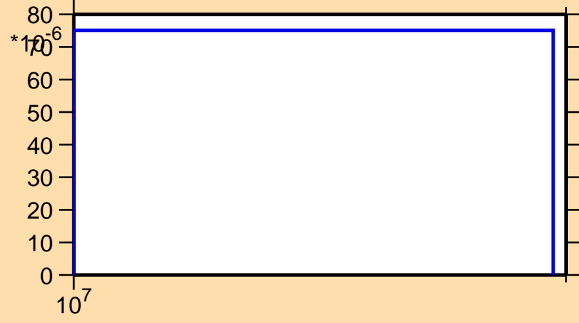
\sigma vs. E for ^{40}\text{Cl}(n,n\alpha)
