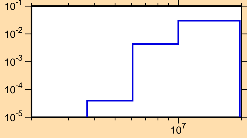
\sigma vs. E for ^{40}\text{Cl}(n,p)
