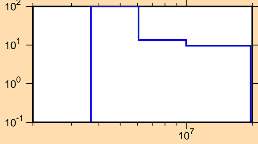
\Delta\sigma/\sigma vs. E for ^{40}\text{Cl}(n,2n)
