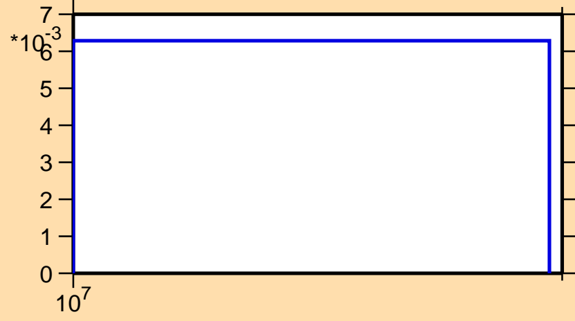
\sigma vs. E for ^{40}\text{Cl}(n,3n)
