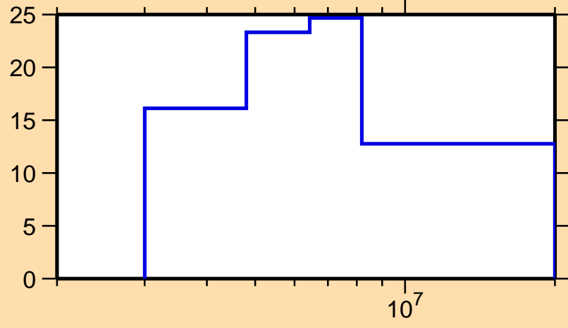
\Delta\sigma/\sigma vs. E for ^{40}\text{Cl}(n,el.)
