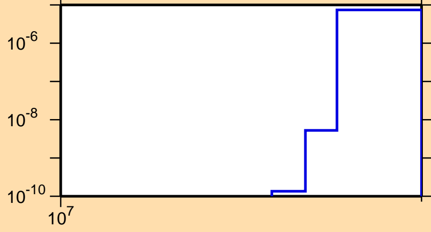
\sigma vs. E for ^{41}\text{Cl}(n,nt)
