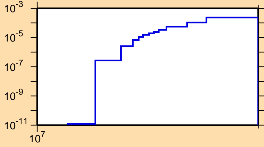
\sigma vs. E for ^{41}\text{Cl}(n,t)
