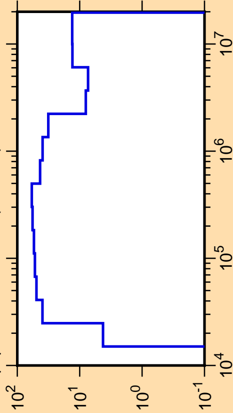
\Delta\mu/\mu vs. E for ^{41}\text{Cl}(\text{mt251})
