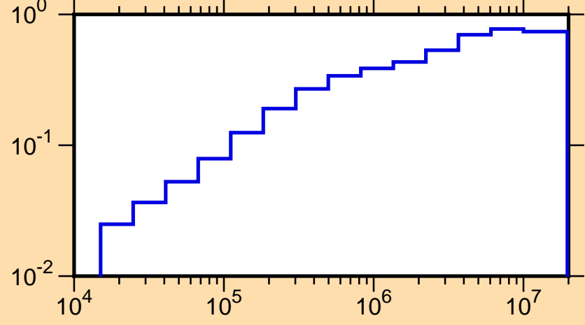
\mu vs. E for ^{41}\text{Cl}(\text{mt251})
