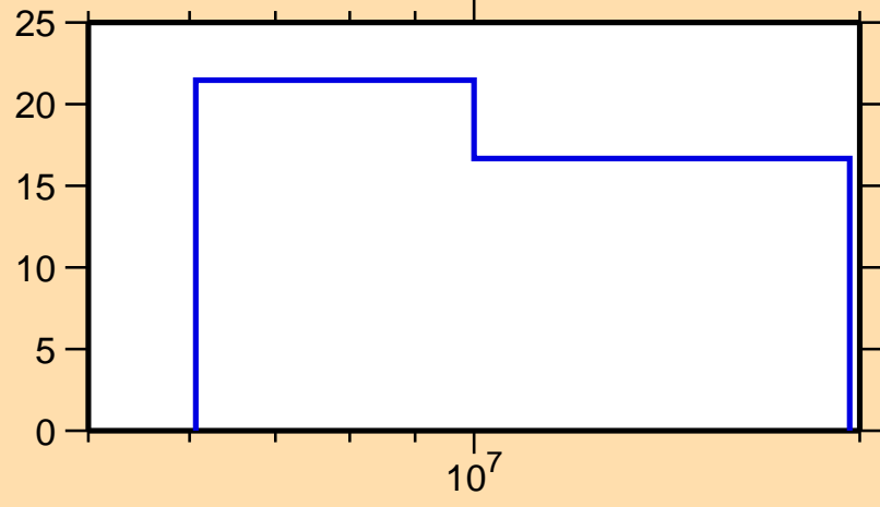
\Delta\sigma/\sigma vs. E for ^{41}\text{Cl}(n,el.)
