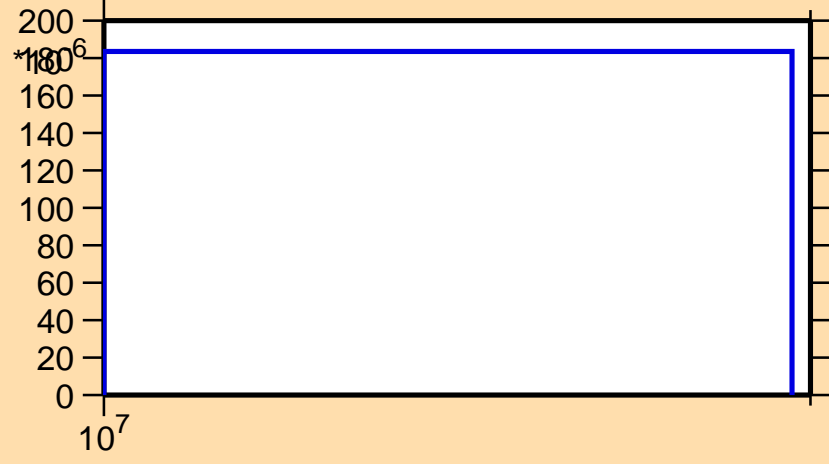
\sigma vs. E for ^{41}\text{Cl}(n,np)
