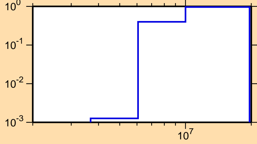
\sigma vs. E for ^{42}\text{Cl}(n,2n)
