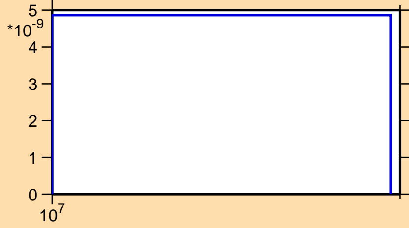
\sigma vs. E for ^{42}\text{Cl}(n,nt)
