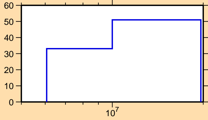
\Delta\sigma/\sigma vs. E for ^{42}\text{Cl}(n,ncont.)
