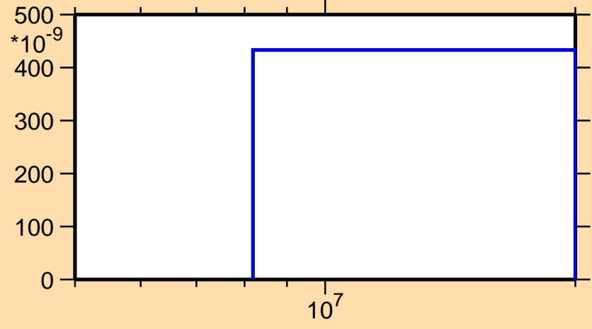
\sigma vs. E for ^{42}\text{Cl}(n,\alpha)
