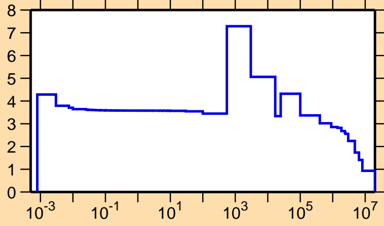
\sigma vs. E for ^{42}\text{Cl}(n,\text{el.})
