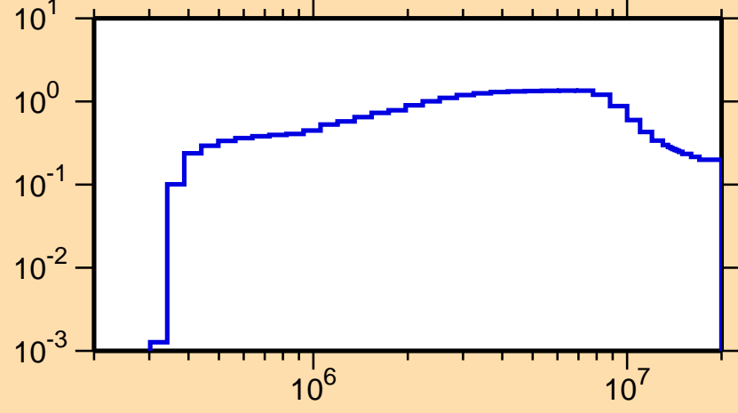
\sigma vs. E for ^{43}\text{Cl}(n,\text{inel.})
