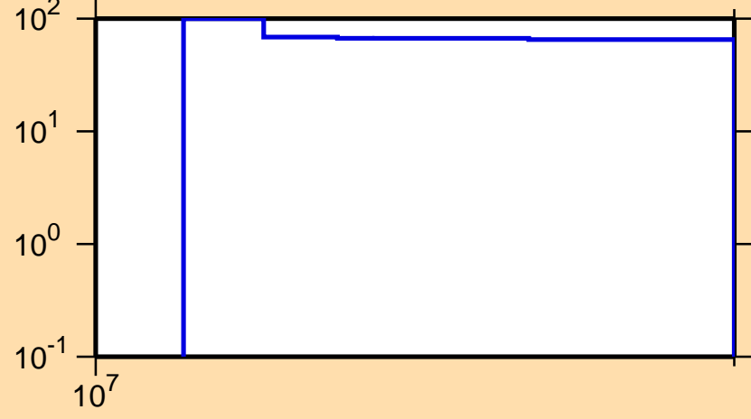
\Delta\sigma/\sigma vs. E for ^{43}\text{Cl}(n,p)
