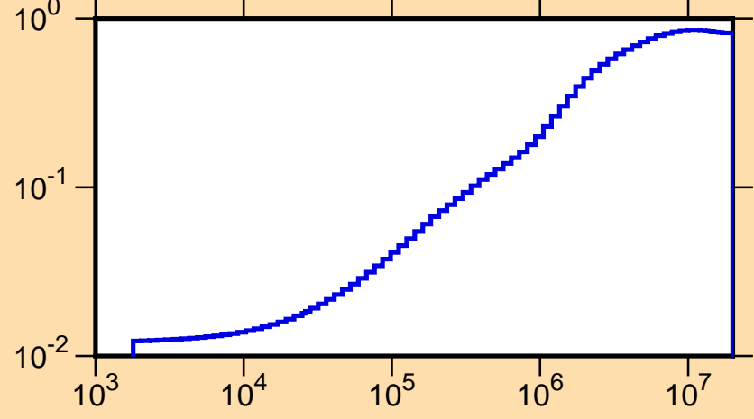
\mu vs. E for ^{56}\text{Co}(\text{mt251})
