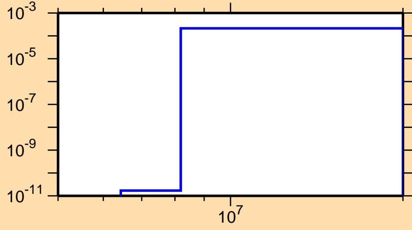
\sigma vs. E for ^{56}\text{Co}(n,t)
