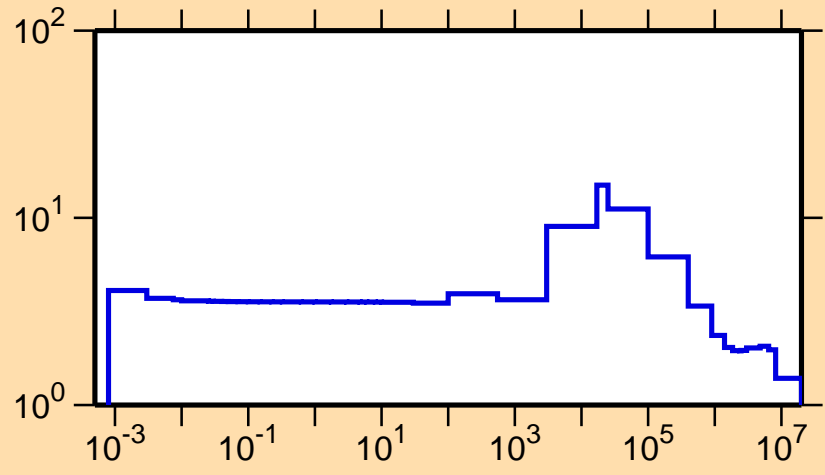
\sigma vs. E for ^{56}\text{Co}(n,\text{el.})
