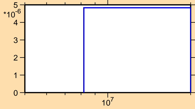
\sigma vs. E for ^{56}\text{Co}(n,\text{nd})
