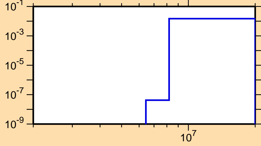
\sigma vs. E for ^{56}\text{Co}(n,p\alpha)
