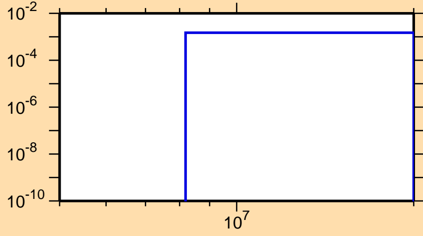
\sigma vs. E for ^{56}\text{Co}(n,\alpha)
