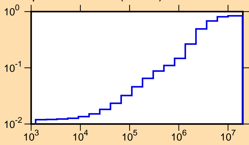
\mu vs. E for ^{57}\text{Co}(\text{mt251})
