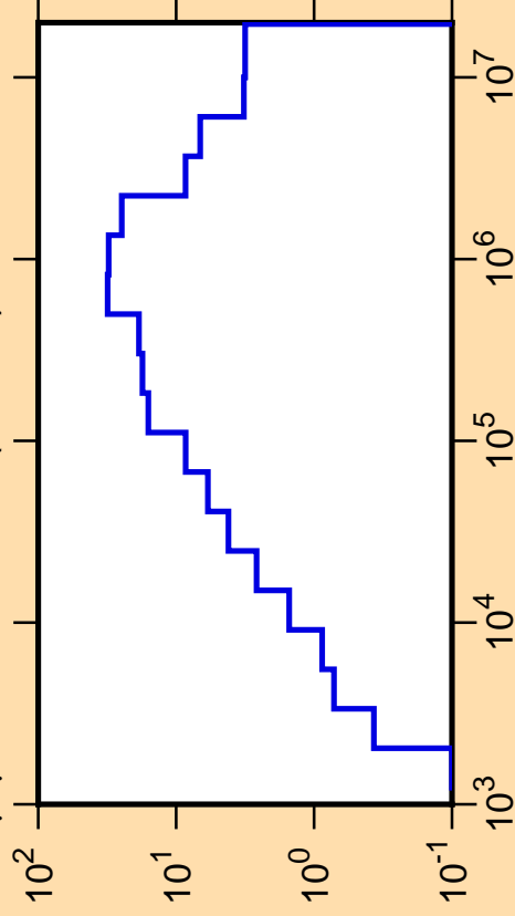
\Delta\mu/\mu vs. E for ^{57}\text{Co}(\text{mt251})
