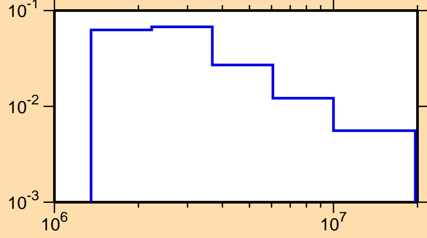
\sigma vs. E for ^{57}\text{Co}(n,n_2)
