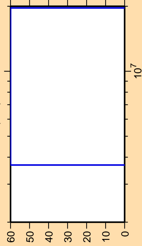
\Delta\sigma/\sigma vs. E for ^{57}\text{Co}(n,d)
