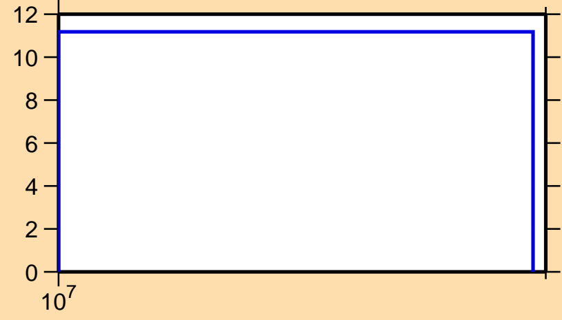
\Delta\sigma/\sigma vs. E for ^{57}\text{Co}(n,el.)
