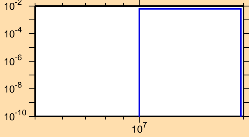
\sigma vs. E for ^{57}\text{Co}(n,\alpha)
