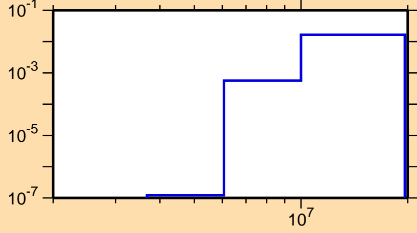
\sigma vs. E for ^{57}\text{Co}(n,d)
