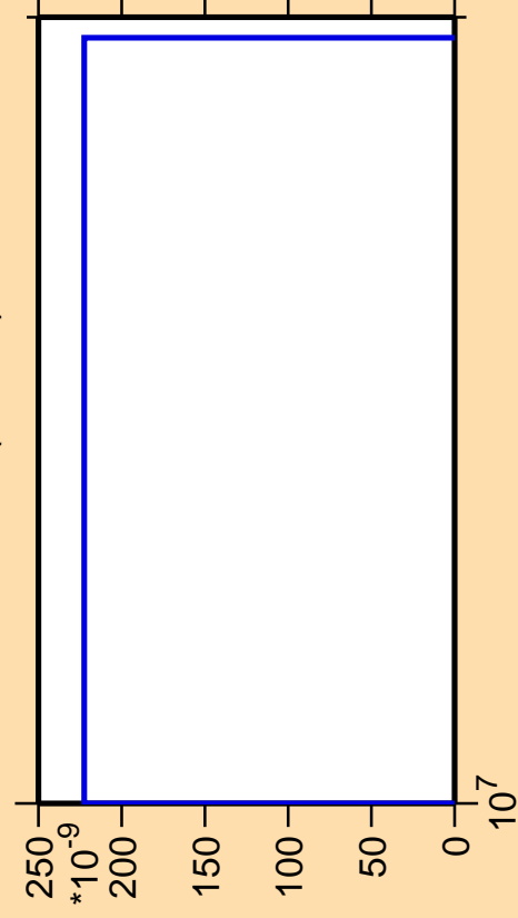
\Delta\sigma/\sigma vs. E for ^{57}\text{Co}(n,2n\alpha)
