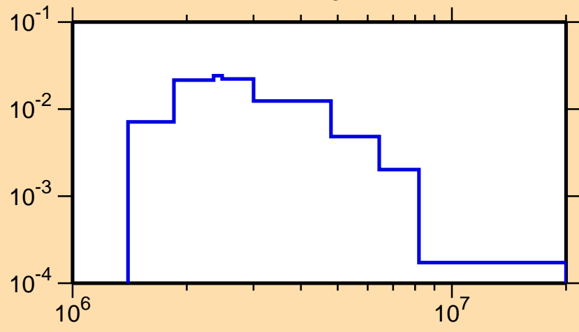
\sigma vs. E for ^{57}\text{Co}(n,n_3)
