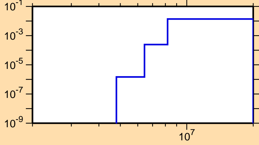
\sigma vs. E for ^{57}\text{Co}(n,d)
