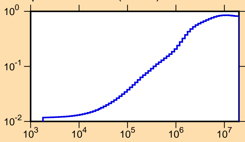
\mu vs. E for ^{58}\text{Co}(\text{mt251})
