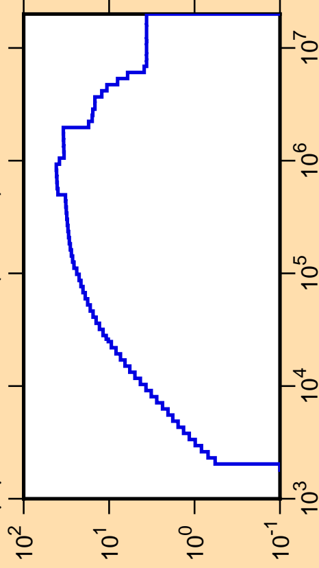
\Delta\mu/\mu vs. E for ^{58}\text{Co}(\text{mt251})
