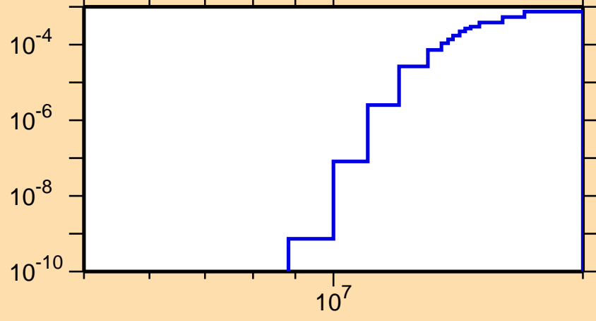
\sigma vs. E for ^{58}\text{Co}(n,p\alpha)
