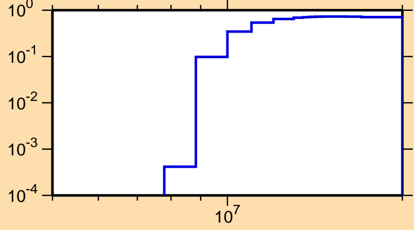
\sigma vs. E for ^{58}\text{Co}(n,2n)
