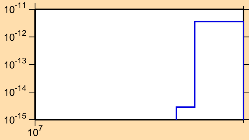
\sigma vs. E for ^{58}\text{Co}(n,\text{pt})
