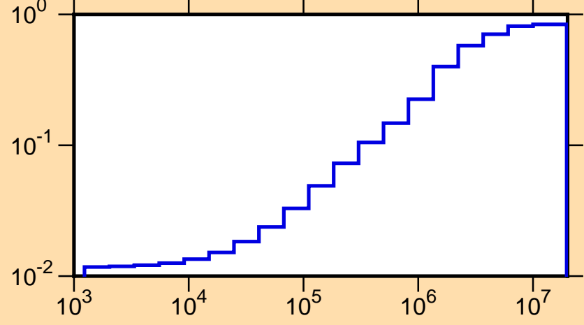
\mu vs. E for ^{58}\text{Co}(\text{mt251})
