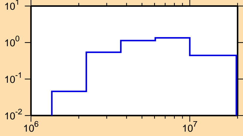
\sigma vs. E for ^{58}\text{Co}(n,n\text{cont.})
