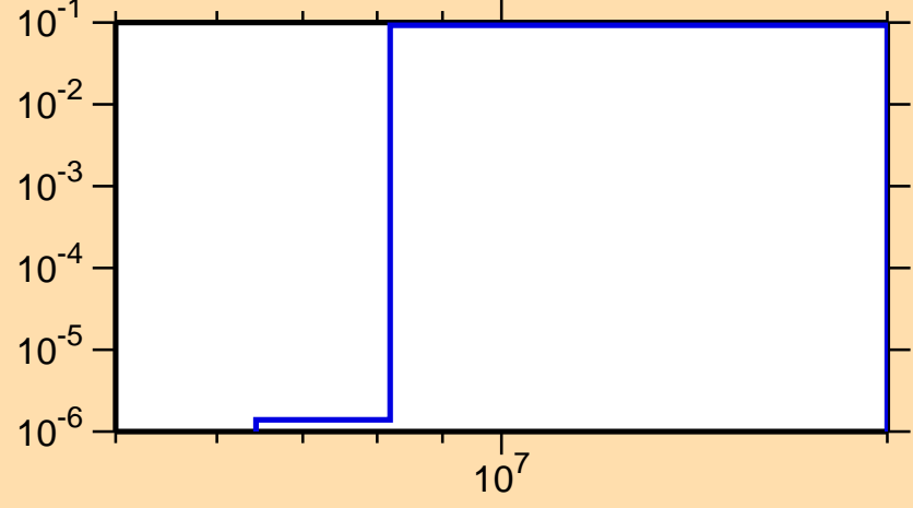
\sigma vs. E for ^{58}\text{Co}(n,np)
