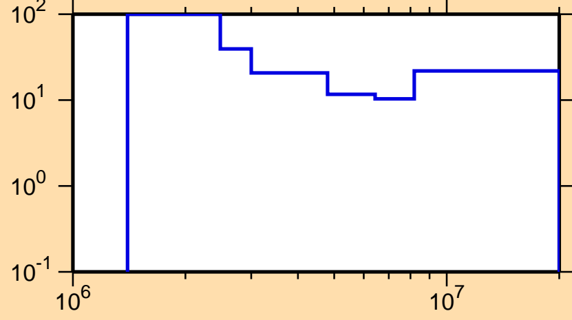
\Delta\sigma/\sigma vs. E for ^{58}\text{Co}(n,n\text{cont.})
