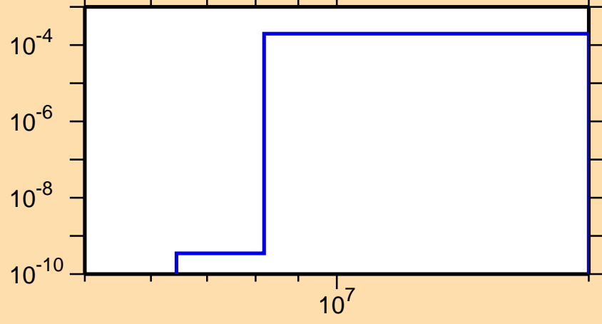
\sigma vs. E for ^{58}\text{Co}(n,t)
