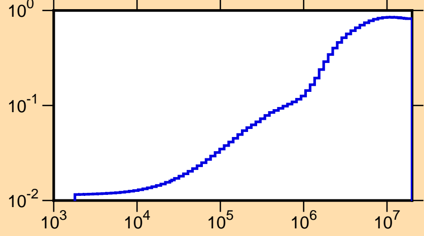
\mu vs. E for ^{59}\text{Co}(\text{mt251})
