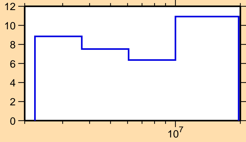
\Delta\sigma/\sigma vs. E for ^{59}\text{Co}(n,n\text{cont.})
