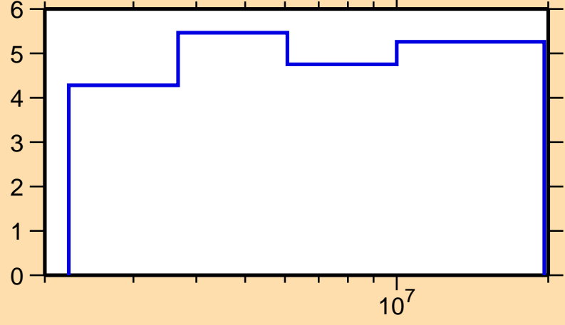
\Delta\sigma/\sigma vs. E for ^{59}\text{Co}(n,n\text{nonel.})
