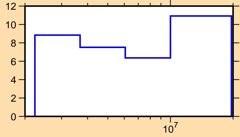
\Delta\sigma/\sigma vs. E for ^{59}\text{Co}(n,ncont.)
