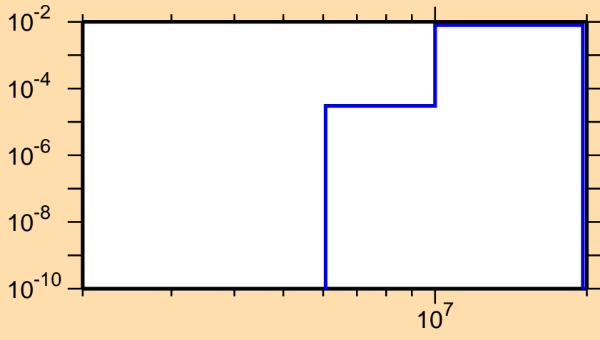
\sigma vs. E for ^{59}\text{Co}(n,d)
