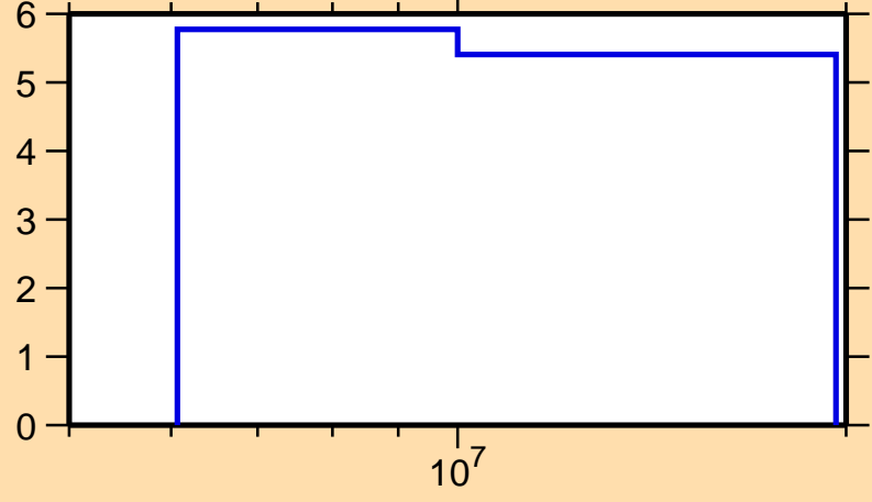
\Delta\sigma/\sigma vs. E for ^{60}\text{Co}(n,\text{nonel.})
