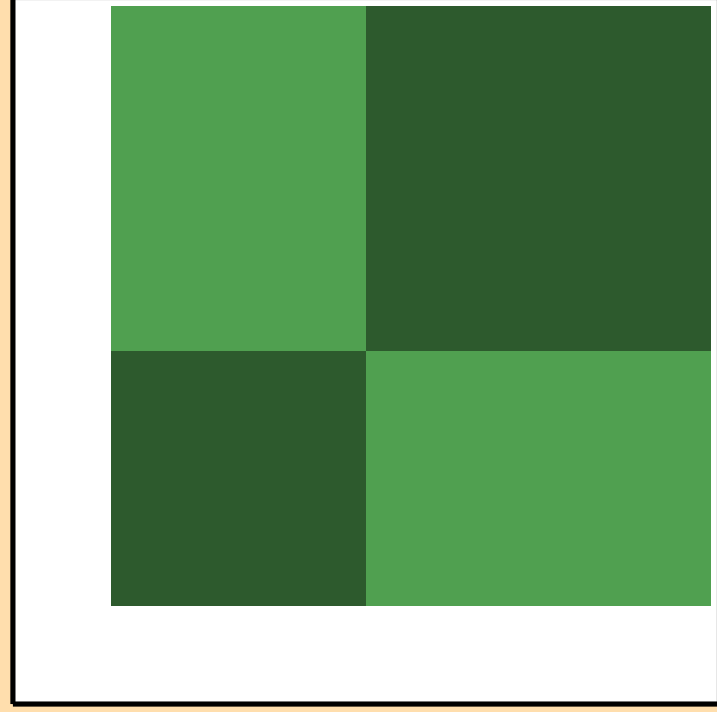
\sigma vs. E for ^{60}\text{Co}(n,t)
