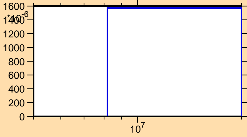
\sigma vs. E for ^{60}\text{Co}(n,\alpha)
