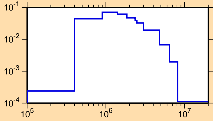
\sigma vs. E for ^{60}\text{Co}(n,n_4)
