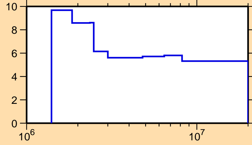
\Delta\sigma/\sigma vs. E for ^{60}\text{Co}(n,n\text{onrel.})
