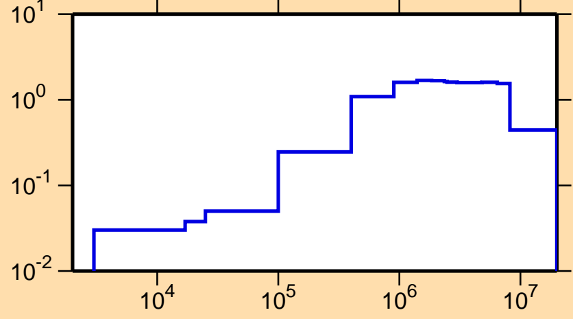
\sigma vs. E for ^{60}\text{Co}(n,\text{inel.})
