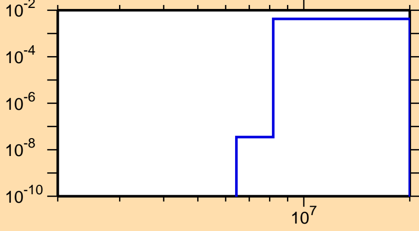
\sigma vs. E for ^{60}\text{Co}(n,d)
