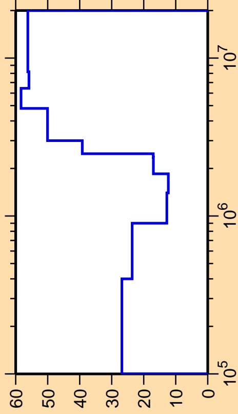
\Delta\sigma/\sigma vs. E for ^{60}\text{Co}(n,n_4)
