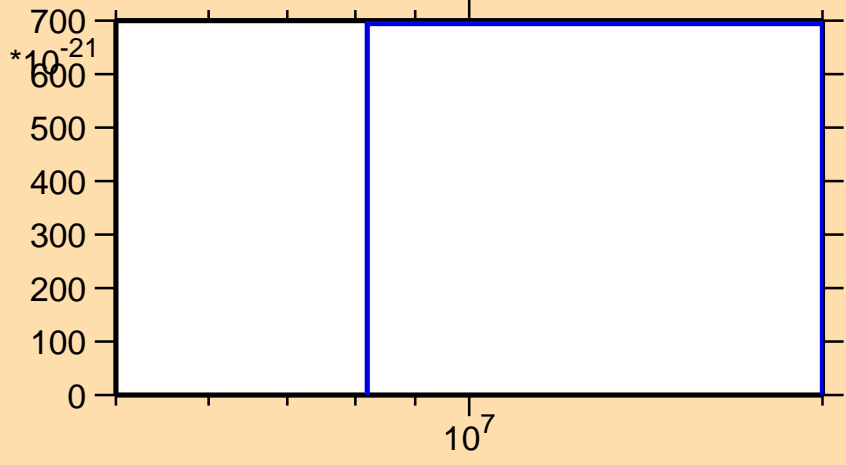
\sigma vs. E for ^{60}\text{Co}(n,pd)
