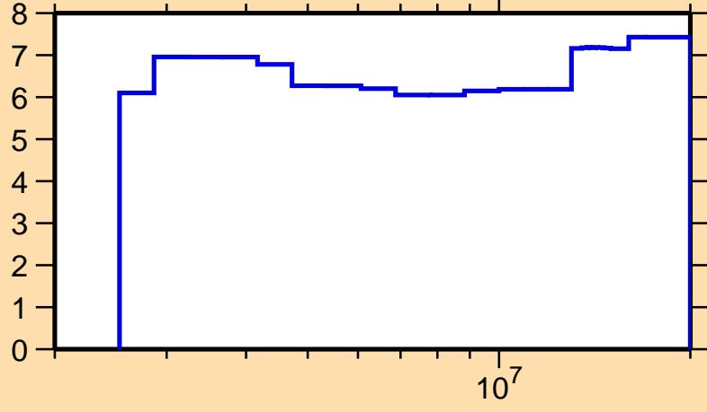
\Delta\sigma/\sigma vs. E for ^{61}\text{Co}(n,n\text{onel.})
