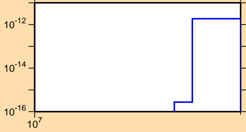
\sigma vs. E for ^{61}\text{Co}(n,\text{He}3)
