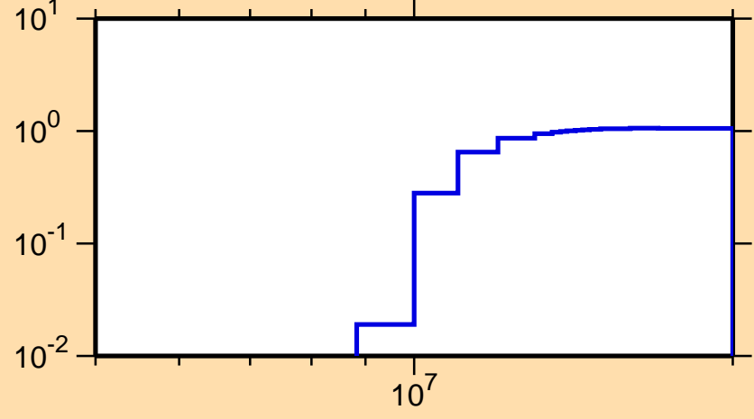
\sigma vs. E for ^{61}\text{Co}(n,2n)
