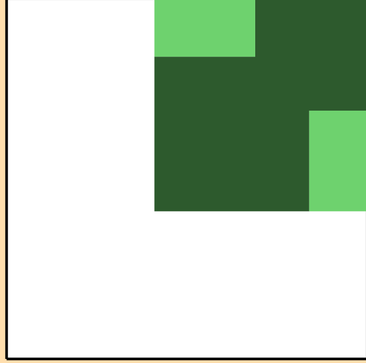
\sigma vs. E for ^{61}\text{Co}(n,np)
