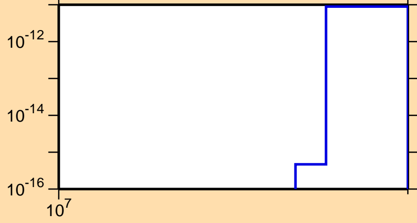
\sigma vs. E for ^{61}\text{Co}(n,p\alpha)
