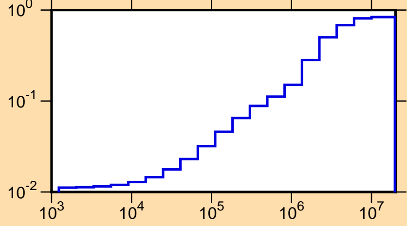
\mu vs. E for ^{61}\text{Co}(\text{mt251})
