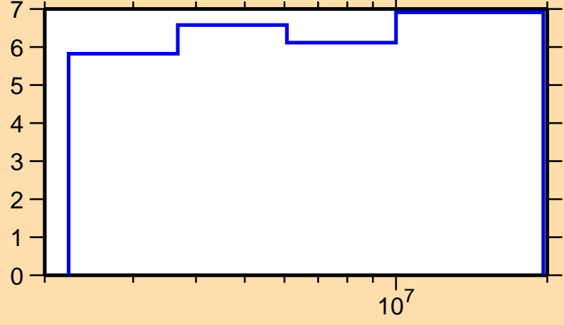
\Delta\sigma/\sigma vs. E for ^{61}\text{Co}(n,n\text{nonel.})
