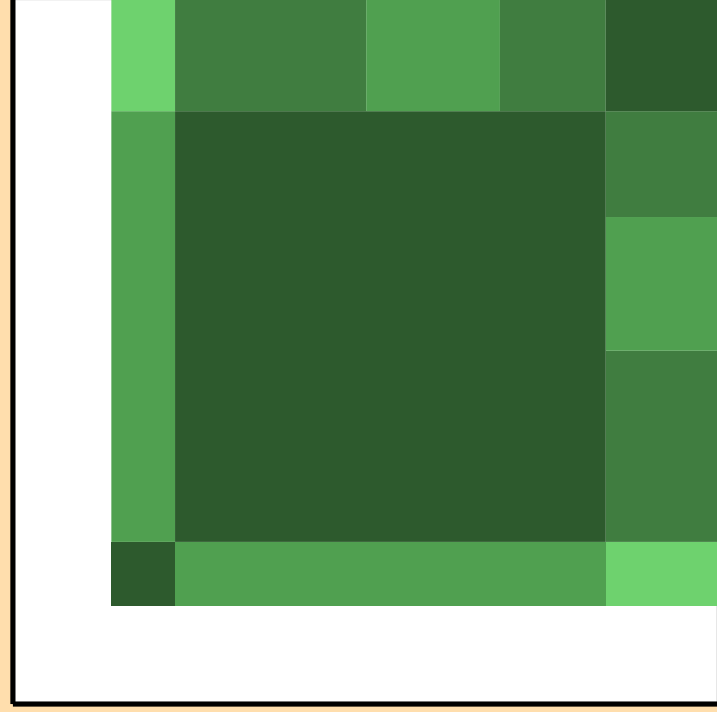
\sigma vs. E for ^{62}\text{Co}(n,2n)
