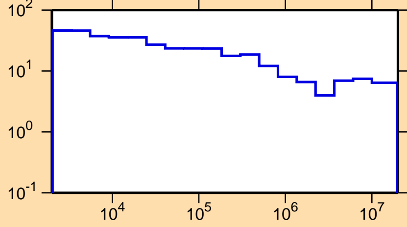
\Delta\sigma/\sigma vs. E for ^{62}\text{Co}(n,\text{nonel.})
