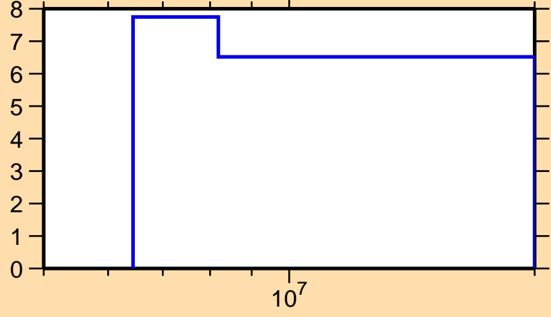
\Delta\sigma/\sigma vs. E for ^{62}\text{Co}(n,\text{nonel.})
