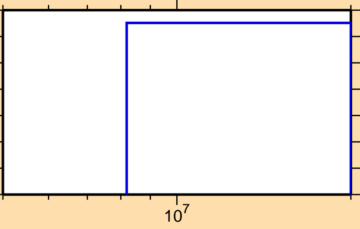
\sigma vs. E for ^{62}\text{Co}(n,\text{nd})
