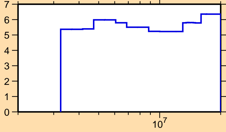
\Delta\sigma/\sigma vs. E for ^{63}\text{Co}(n,nonel.)
