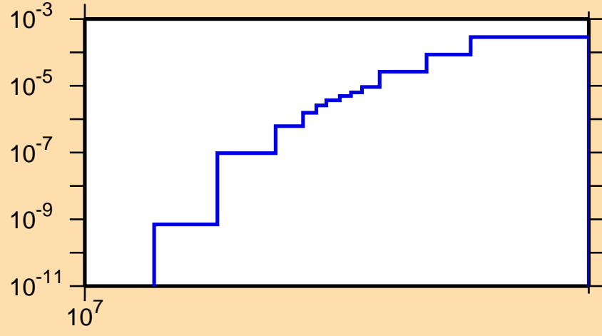
\sigma vs. E for ^{63}\text{Co}(n,t)
