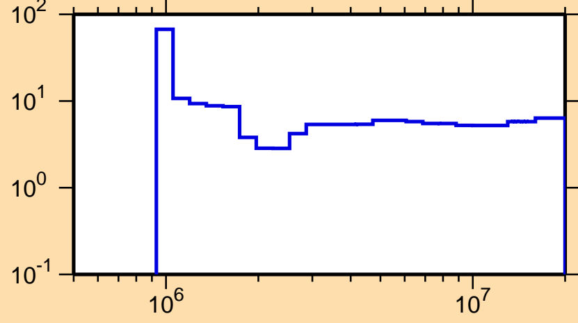
\Delta\sigma/\sigma vs. E for ^{63}\text{Co}(n,\text{nonel.})
