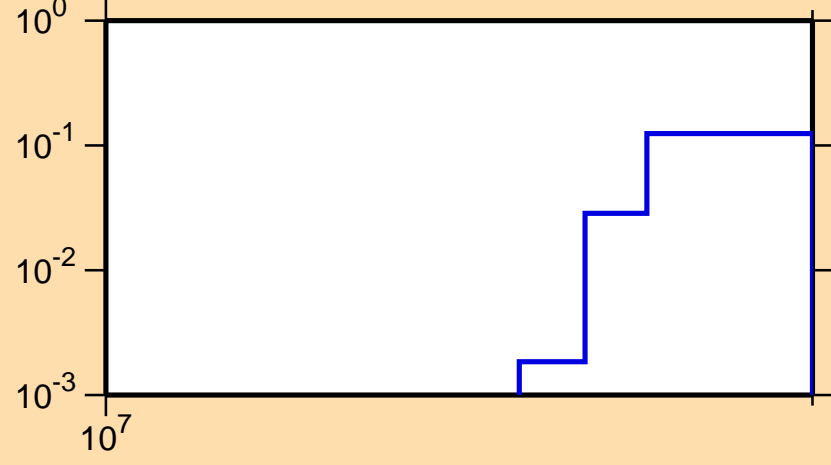
\sigma vs. E for ^{63}\text{Co}(n,3n)
