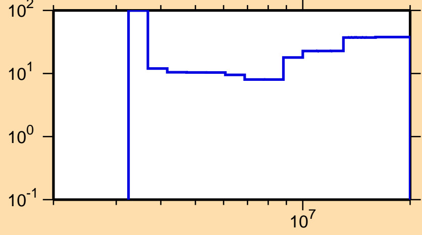
\Delta\sigma/\sigma vs. E for ^{63}\text{Co}(n,ncont.)
