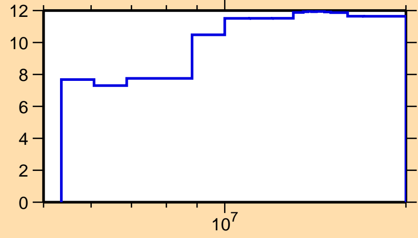
\Delta\sigma/\sigma vs. E for ^{63}\text{Co}(n,el.)
