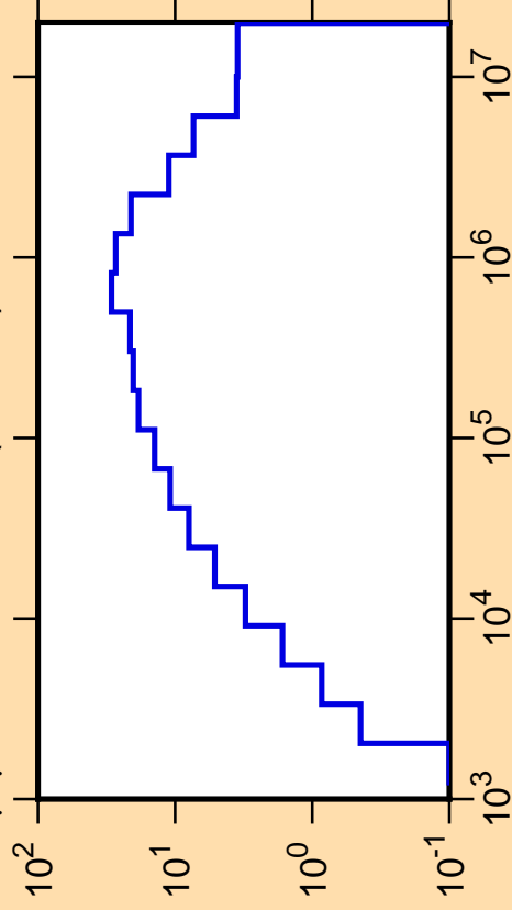
\Delta\mu/\mu vs. E for ^{63}\text{Co}(\text{mt251})
