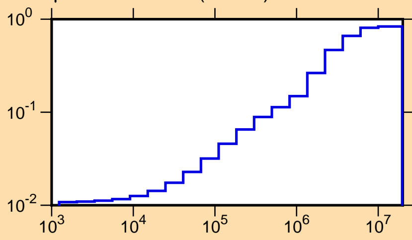
\mu vs. E for ^{63}\text{Co}(\text{mt251})
