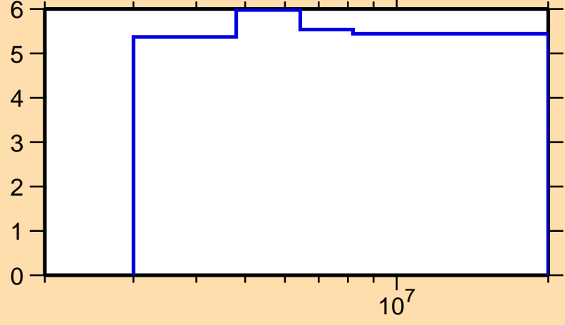
\Delta\sigma/\sigma vs. E for ^{63}\text{Co}(n,n\text{nonel.})
