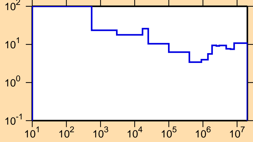
\Delta\sigma/\sigma vs. E for ^{63}\text{Co}(n,\text{el.})
